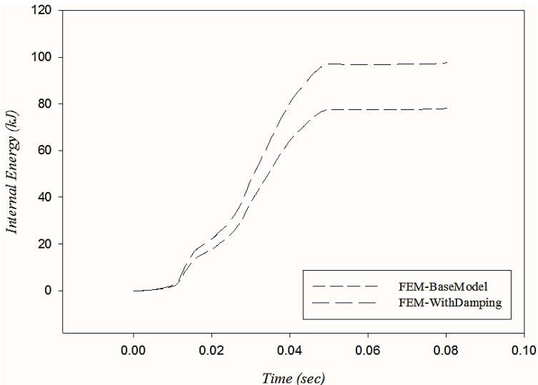
Fig17. Time histories of the internal energy when considering/neglecting the structural damping of the body.
