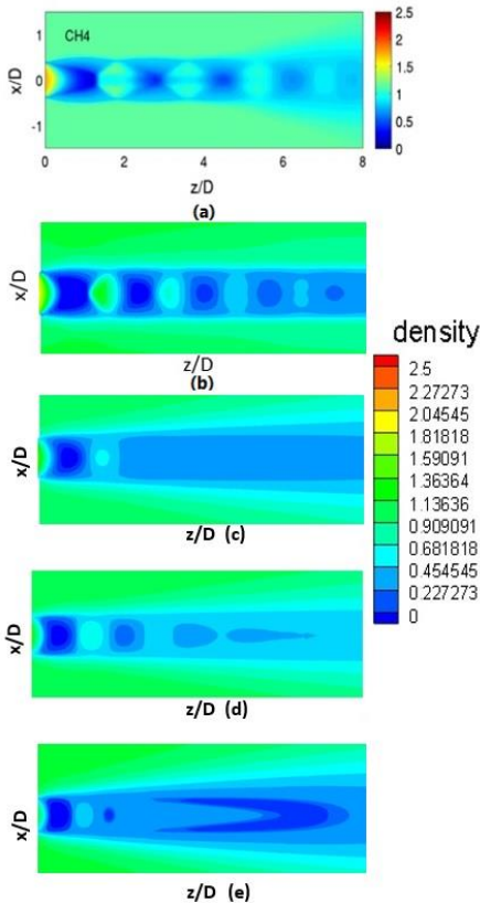
Figure 5 Contour of density at 0.5 ms for a: Vuorinen et al.'s study[12] b: this study with LES turbulence model - c: this study with standard k - \varepsilon turbulence model - d: this study with RNG k - \varepsilon turbulence model - e: this study with SST k - \omega turbulence model
