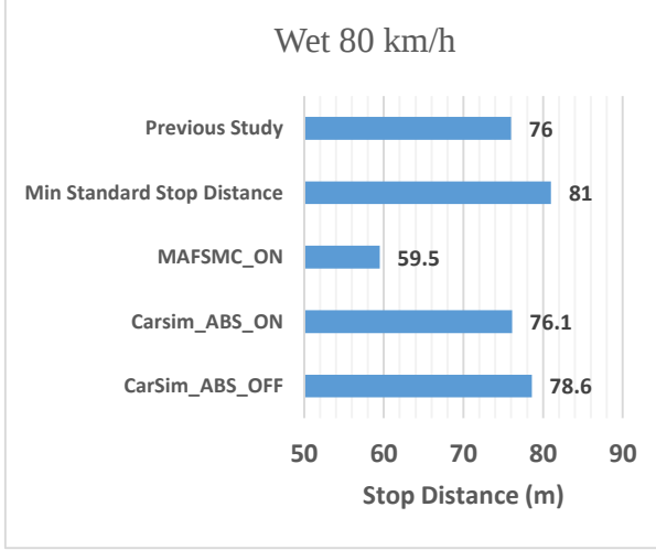
Figure40: Comparison of Brake Distance in different situations
