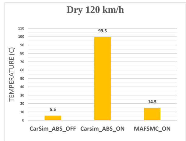
Figure30: Comparison of Brake Rotor Temperature in different situation (No exceed)
