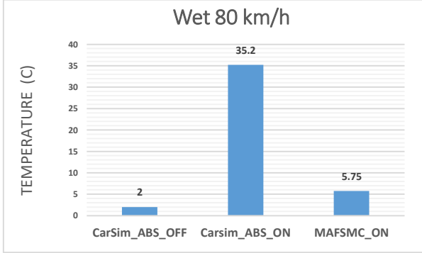
Figure41: Comparison of Brake Rotor Temperature in different situation (No exceed)
