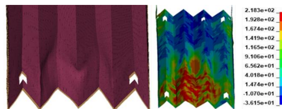
Fig.7. Schematic illustration of multi-V-shaped hull deformation
