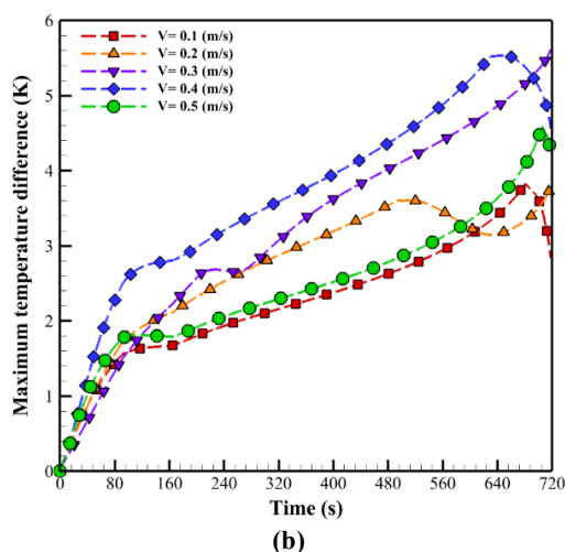
Figure 4: distribution diagram of (a) T_{\max} and (b) \Delta T_{\max} with different speed values
