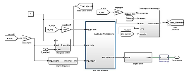
Figure 8: Internal Combustion Engine (ICE) Block Diagram.
