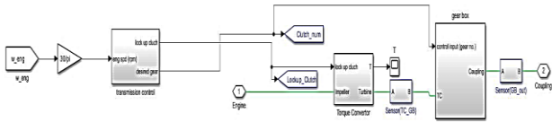
Figure 9: Gearbox Control block diagram.
