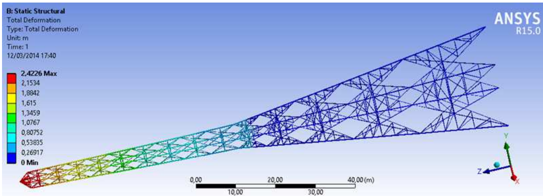
Figure 15. Total deflection due to loads in ANSYS®
