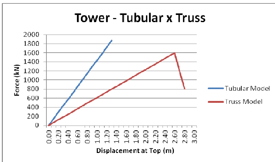
Figure 5. Load versus displacement curve for the wind to 0°
