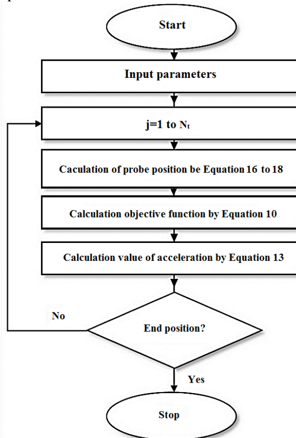
Figure 1. CFO algorithm
