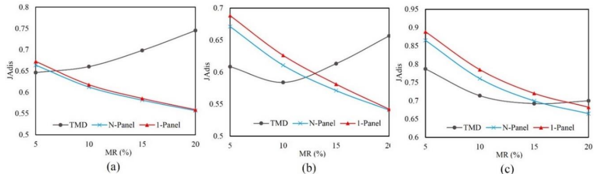
Figure 11. Optimum values of drift objective function for different MRs (a) 10-story model (b) 20-story model (c) 30-story model
