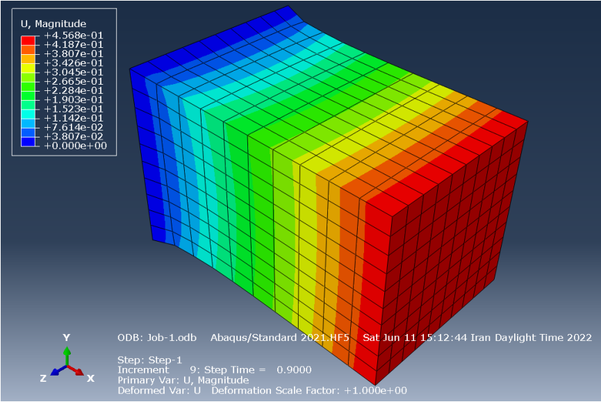
Figure 13. The magnitude displacement field of the ABAQUS.
