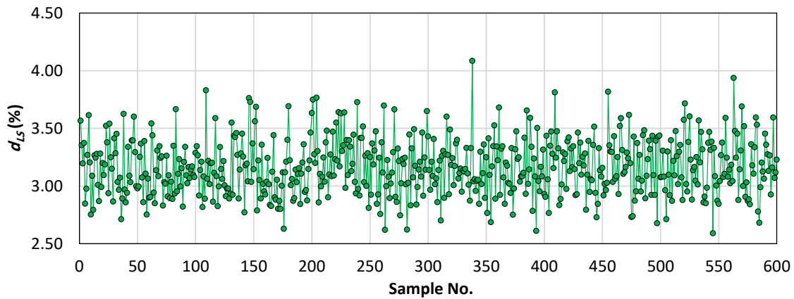
Figure 16. Maximum inter-story drift ratios at LS level for 10-story steel MRF
