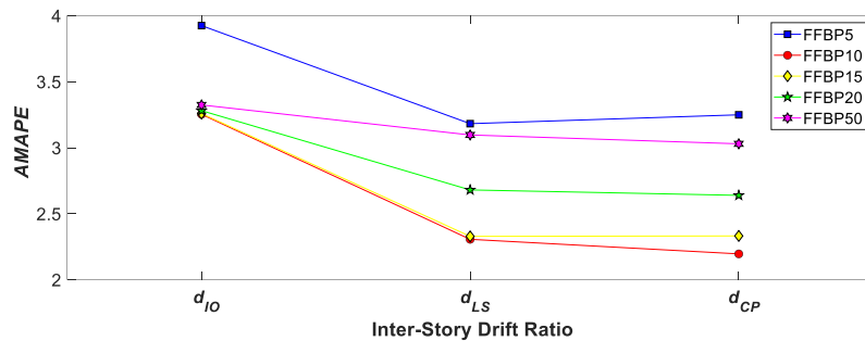
Figure 10. AMAPE of inter-story drift ratios predicted by NN models for 5-story steel SMF
