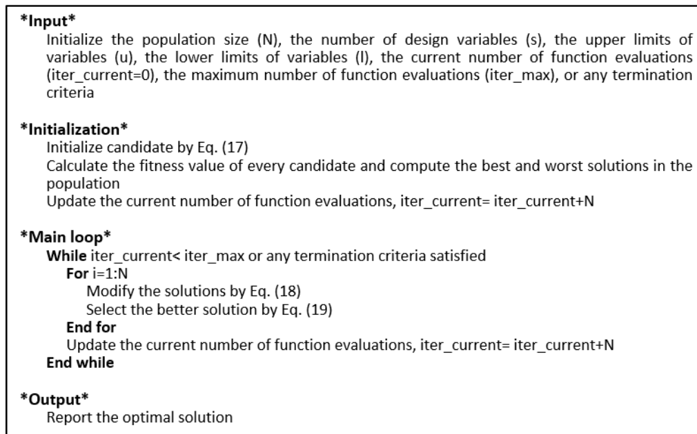
Figure 1: Pseudocode of an unconstrained Jaya optimization algorithm
