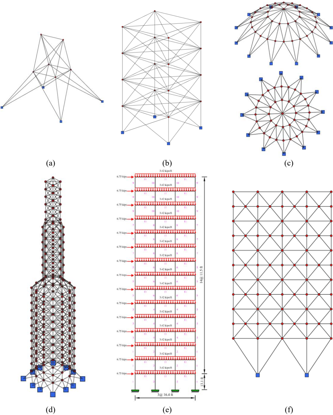
Figure 3: Benchmark structures: (a) 25-bar truss, (b) 72-bar truss, (c) 120-bar dome, (d) 942-bar truss, (e) 3-bay, 15-story frame, (f) 200-bar truss
