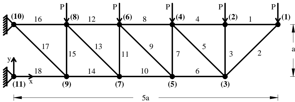
Figure 6. Eighteen-bar truss structure, a = 250 in
