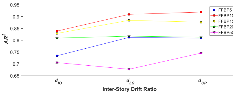
Figure 12. AR^2 of inter-story drift ratios predicted by NN models for 5-story steel SMF
